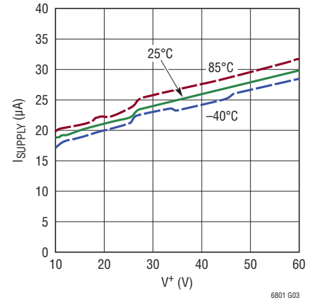
Supply Current, Idle Mode
