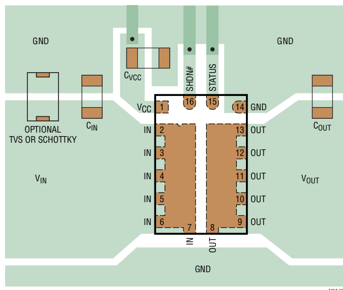
Figure 4. Recommended Layout
