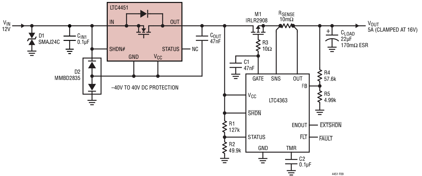
Figure 9. Overvoltage Protector and Ideal Diode Blocks Reverse Input Voltage
