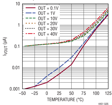
OUT Reverse Leakage vs Temperature
