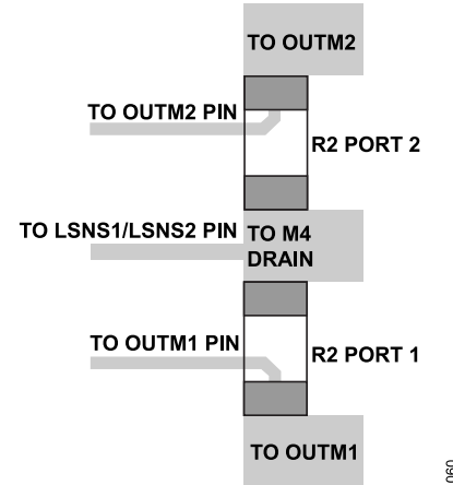
Figure 60. Shared LSNS1/LSNS2 and OUTM1 and OUTM2 Pins Example Kelvin Sense Layout
