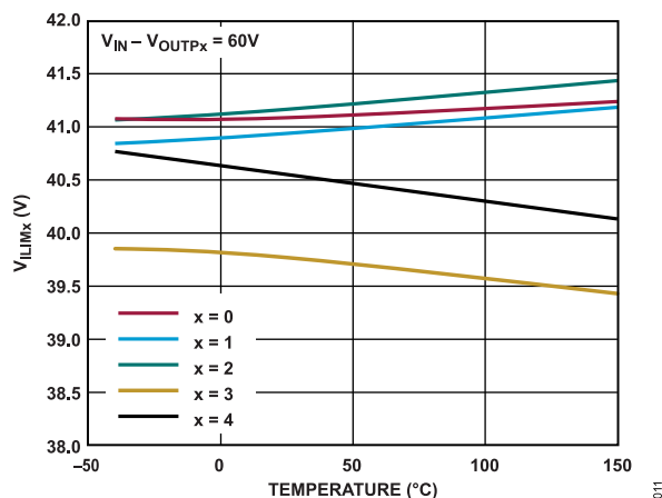
Figure 11. V_{ILIMx} vs. Temperature, V_{IN} - V_{OUTPx} = 60\text{V}
