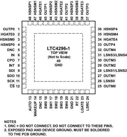
Figure 3. Pin Configuration
