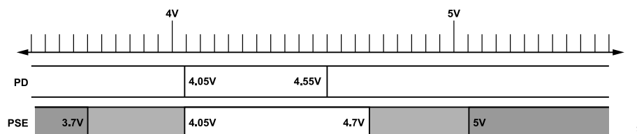
Figure 48. IEEE 802.3bu Signature Voltage Range
