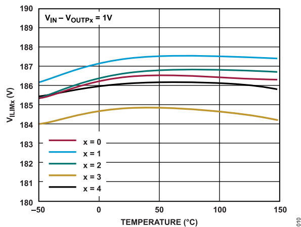
Figure 10. V_{ILIMx} vs. Temperature, V_{IN} - V_{OUTPx} = 1\text{V}
