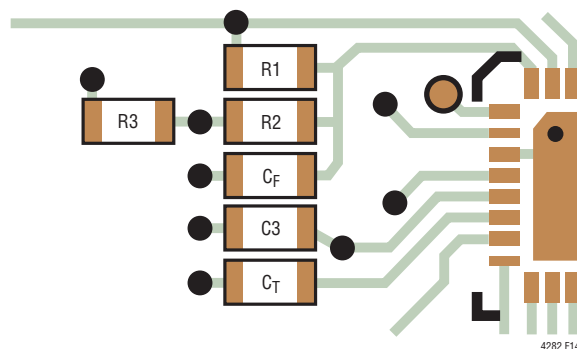
Figure 14. Recommended Layout
