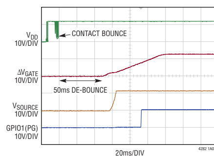
Start-Up Waveforms
