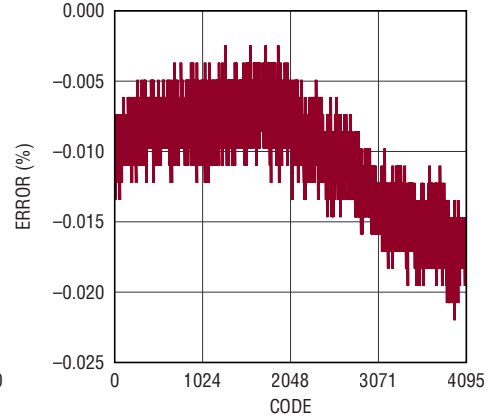
ADC Total Unadjusted Error vs Code (TUE vs Code)
