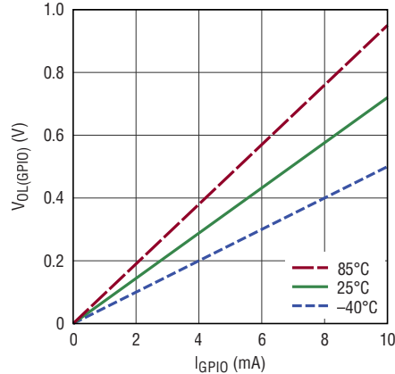
GPIO Pin Output Low Voltage vs Load ( V_{OL(GPIO)} vs I_{GPIO} )
