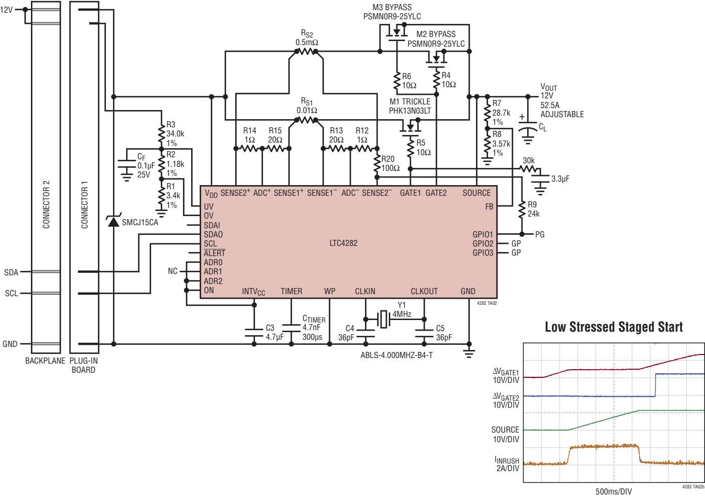
Low Stress, Staged Start 12V, 50A Application
