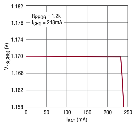
Load Regulation of Regulated Feedback Voltage
