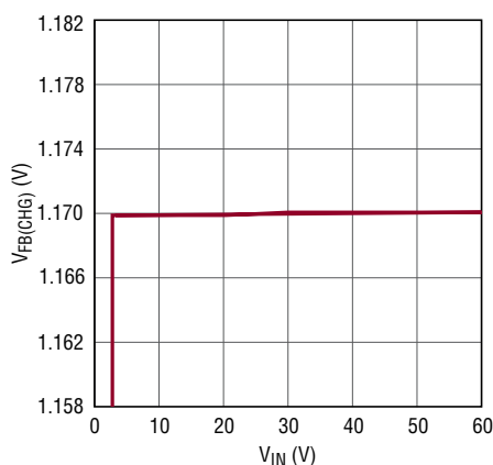
Regulated Feedback Voltage vs V_{IN}
