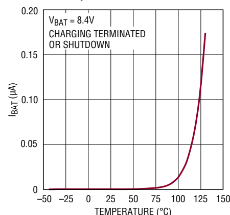
Battery Quiescent Current vs Temperature
