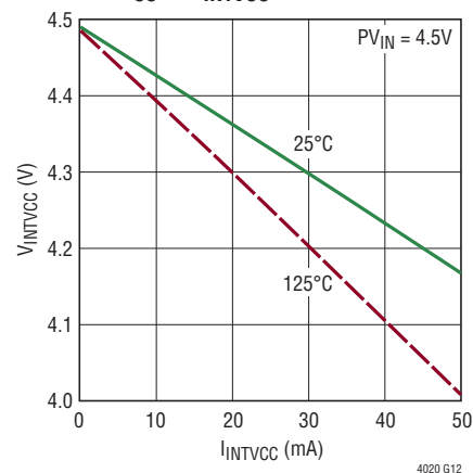
BST Refresh Regulator Dropout V_{INTVCC} vs I_{INTVCC}
