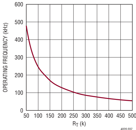
Figure 7. R_T vs Operating Frequency
