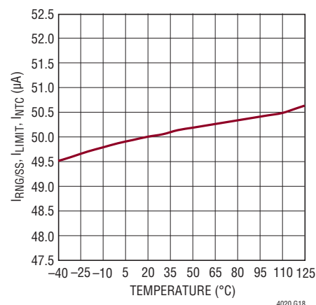
I_{RNG/SS} , I_{LIMIT} , I_{NTC} vs Temperature
