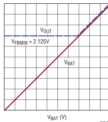
Figure 13. Instant-On DC/DC Converter Output vs Battery Voltage Characteristics
