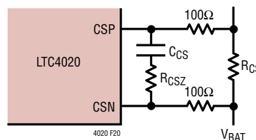
Figure 20. CSN/CSP Ripple Suppression
