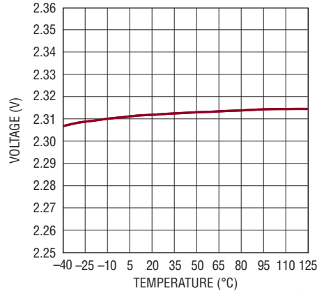
V_{\text{FLOAT(LEAD-ACID)}} Reference vs Temperature
