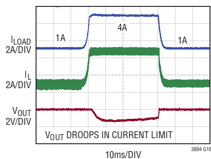
Overcurrent Protection
