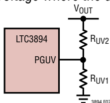
Figure 7. Programmable Power Good UV
