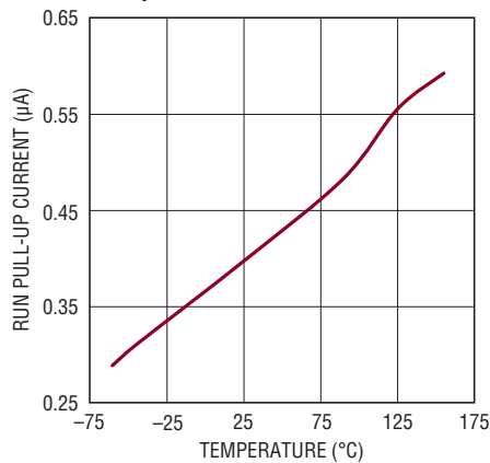
RUN Pin Pull-Up Current Over Temperature
