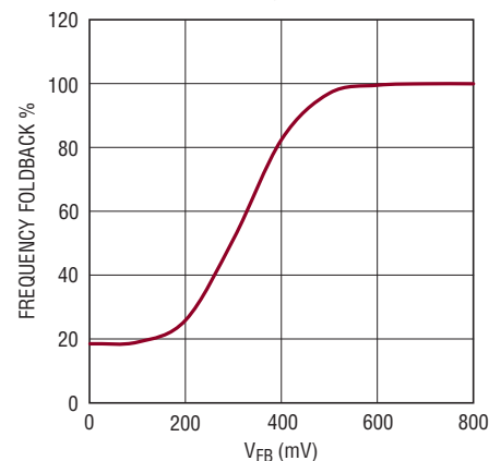
Frequency Foldback % Over Feedback Voltage
