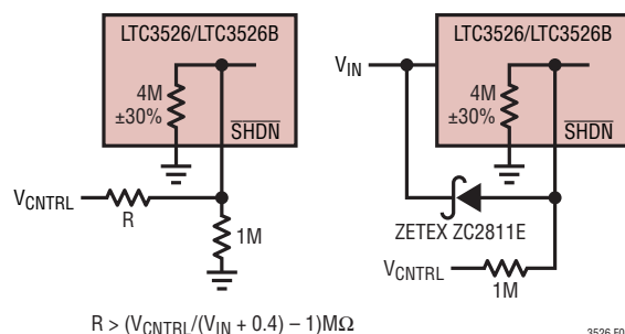
Figure 1. Recommended Shutdown Circuits when Driving \overline{\text{SHDN}} above V_{IN}
