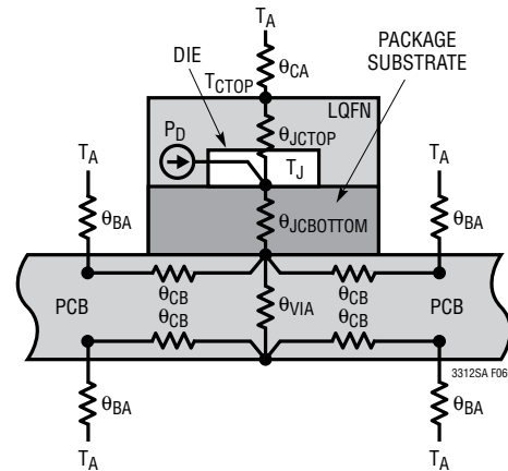
Figure 6. Multi-Layer PCB with Thermal Vias Acts as a Heat Sink
