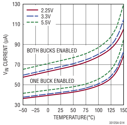
PV IN Quiescent Current, Burst Mode Operation, Sleeping
