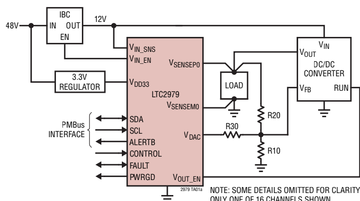
16-Channel PMBus Power System Manager
