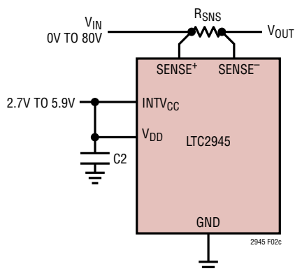
(c) Power from Low Voltage Secondary Supply
