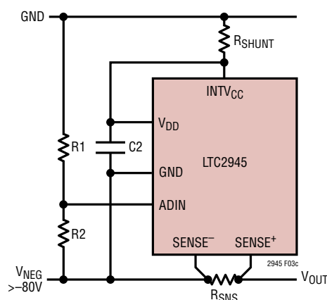
(c) Power Through Low-Side Shunt Regulator in Low-Side Current Sense Topology
