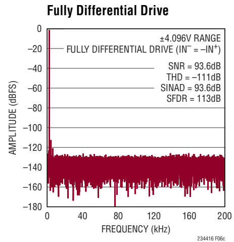
Figure 6c. IN^+/IN^- = -1\text{dBFS} 2kHz Fully Differential Sine, Common Mode = 2.5V, 32k Point FFT, f_{\text{SAMPL}} = 400\text{kps} . Circuit Shown in Figure 6a with LT6237 Amplifiers, R_{\text{FILT}} = 24.9\Omega , C_{\text{FILT}} = 1\text{nF}
