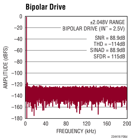
Figure 6d. IN^+ = -1\text{dBFS} 2kHz Bipolar Sine, IN^- = 2.5\text{V} , 32k Point FFT, f_{\text{SAMPL}} = 400\text{kps} . Circuit Shown in Figure 6a with LT6237 Amplifiers, R_{\text{FILT}} = 24.9\Omega , C_{\text{FILT}} = 1\text{nF}
