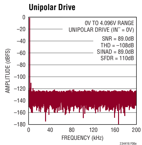
Figure 6e. IN^+ = -1\text{dBFS} 2kHz Unipolar Sine, IN^- = 0\text{V} , 32k Point FFT, f_{\text{SAMPL}} = 400\text{kps} . Circuit Shown in Figure 6a with LT6237 Amplifiers, R_{\text{FILT}} = 24.9\Omega , C_{\text{FILT}} = 1\text{nF}
