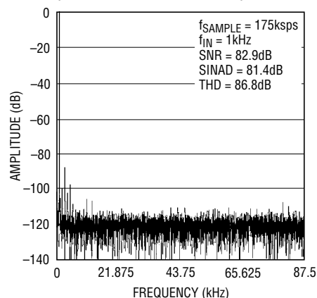
4096 Points FFT Plot ( V_{DD} = 2.7V , Internal REF)
