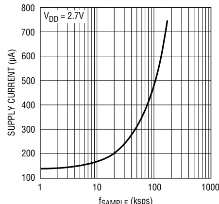
Supply Current vs f_{SAMPLE} (LTC1863L/LTC1867L)
