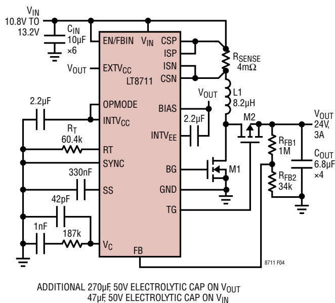
Figure 4. Boost Converter—The Component Values Given are Typical Values for a 400kHz, 12V to 24V/3A Boost
