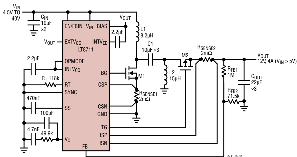
200kHz, 4.5V–40V Input to 12V/4A SEPIC
