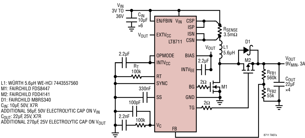
Boost Pre-Regulator for Automotive Stop-Start/Idle
