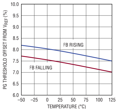
PG Thresholds Above V_{REF}
