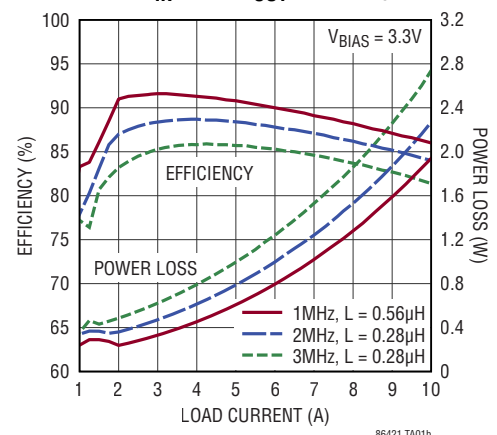
12V IN to 1.2V OUT Efficiency
