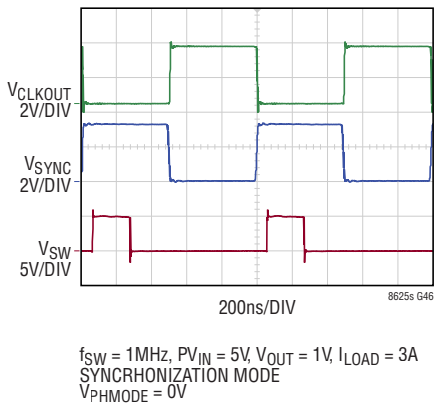
CLKOUT Waveforms
