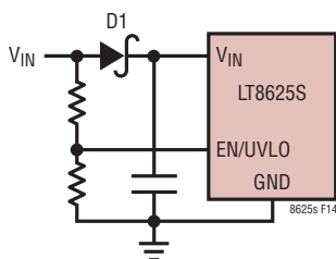
Figure 14. Reverse V_{IN} Protection
