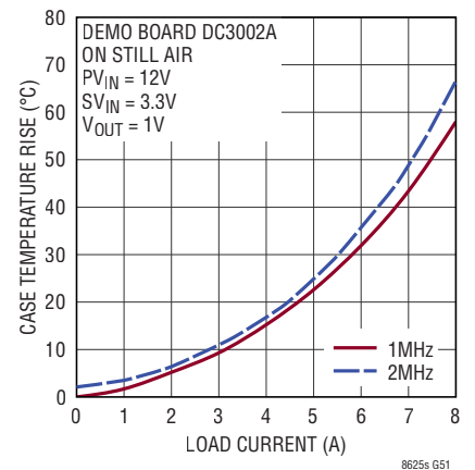
LT8625S Case Temperature Rise
