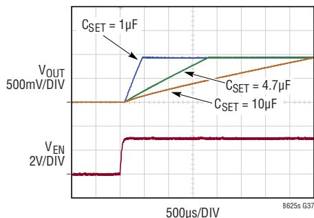
Soft-Start Waveforms
