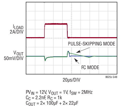
Transient Response: Load Current Stepped from 100mA to 3.1A
