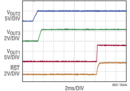
Start-Up Sequence
