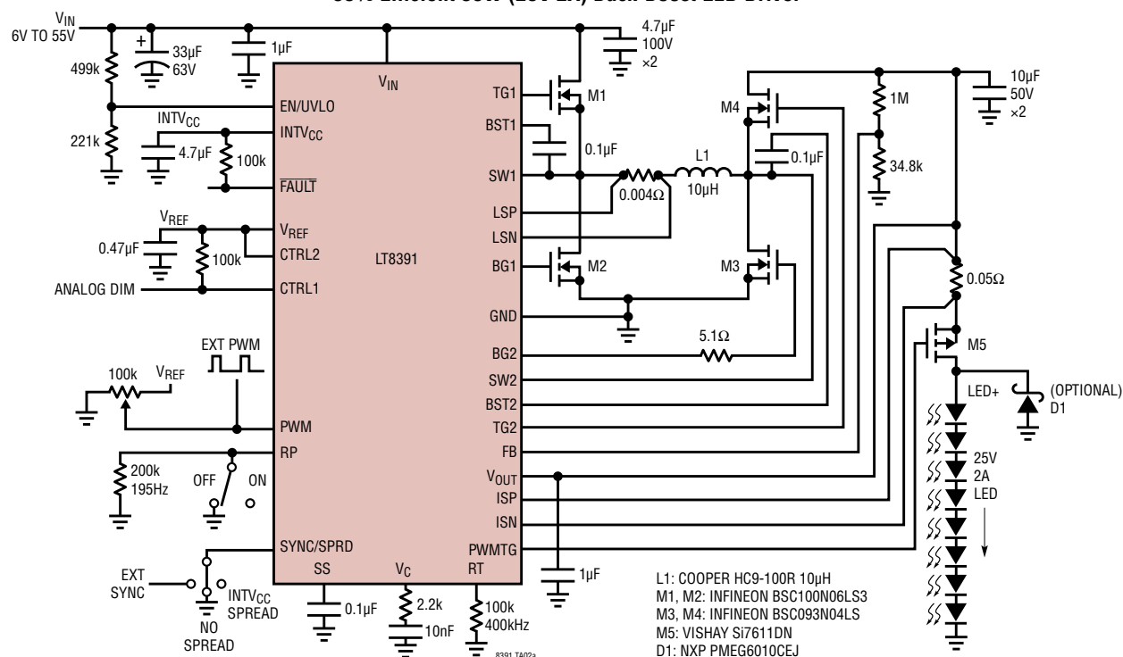
100Hz 1000:1 External PWM Dimming ( V_{IN} = 36V )
