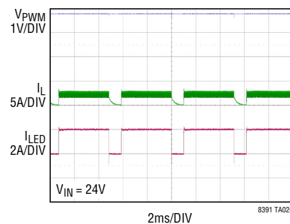
195Hz 80% Internal PWM Dimming ( V_{PWM} = 1.8V )
