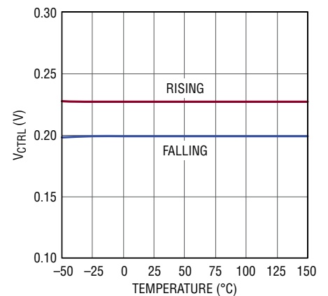
CTRL1/CTRL2 Dim-Off Threshold
