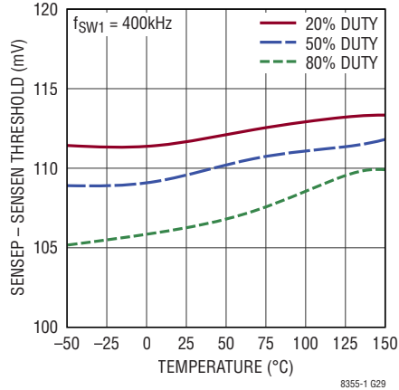
SENSE – SENSEN Current Limit vs Temperature
