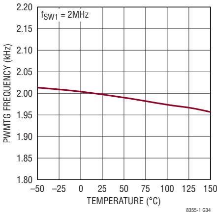
PWMTG Frequency vs Temperature
