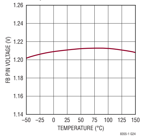
Output Voltage Regulation vs Temperature
