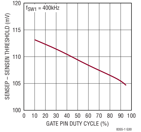
SENSE – SENSEN Current Limit vs Duty Ratio
