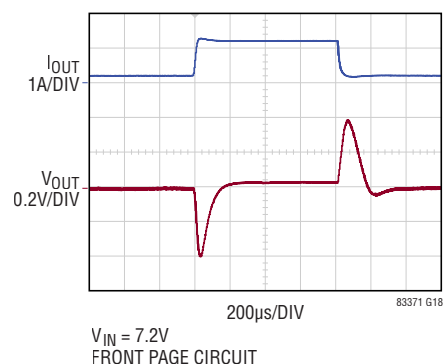
LT8337 Transient Response, Burst Mode Operation
