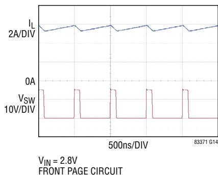
Switching Waveforms, Current Limit at 82% Duty Cycle
