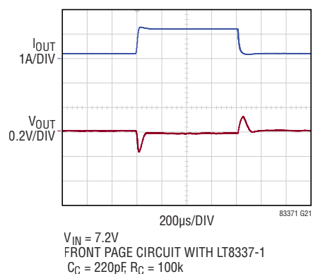
LT8337-1 Transient Response, Burst Mode Operation
