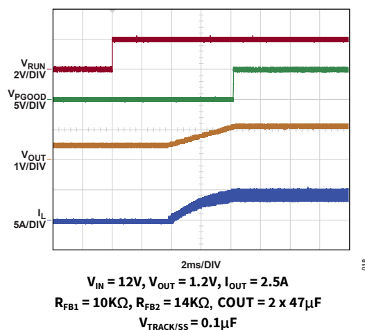
Figure 17. Start-Up Waveform (with Prebiased Output)
