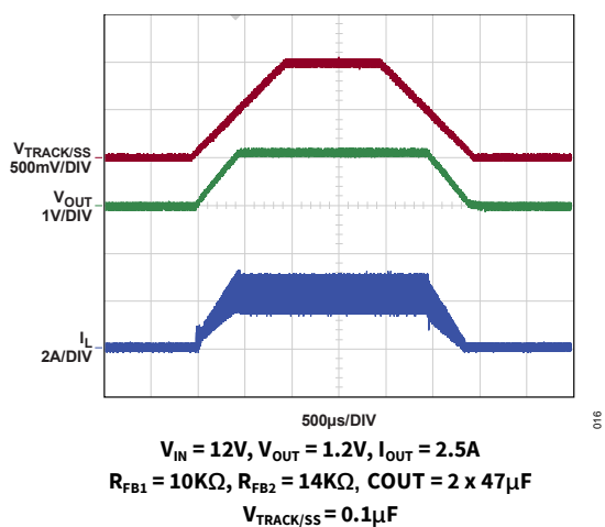
Figure 18. Output Tracking
