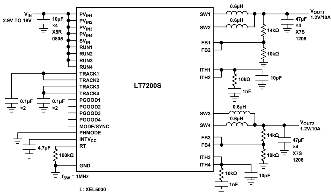
Figure 42. Dual 1.2V, 10A/10A Buck Regulator
