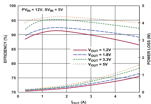
Figure 2. Efficiency and Power Loss (1MHz)
