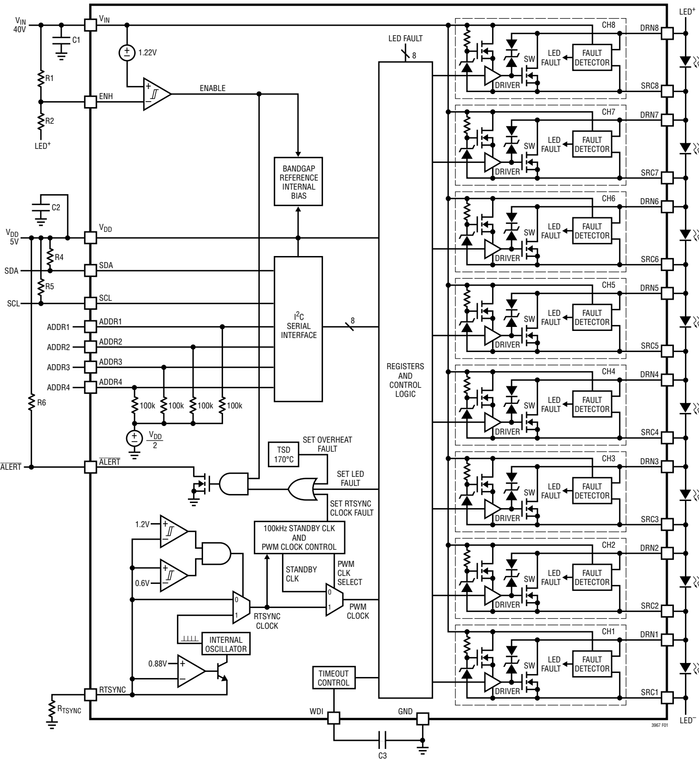
Figure 1. Block Diagram
