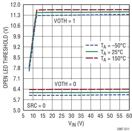
Open LED Threshold vs V_{IN} , for SRC = 0V
