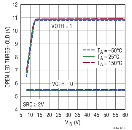
Open LED Threshold vs V_{IN} , for SRC \geq 2V
