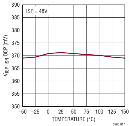
V_{ISP-ISN} Threshold vs Temperature Overcurrent Protection
