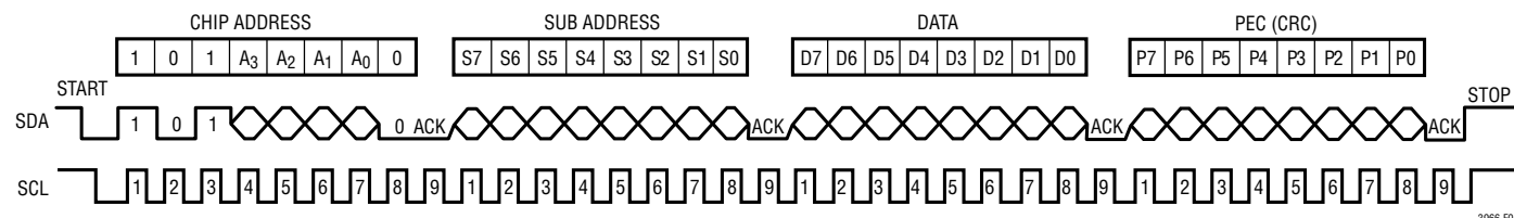
Figure 1. I²C Write Transaction with PEC
