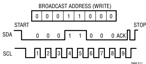
Figure 11. I 2 C Broadcast Write
