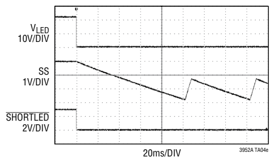
LED Dead Short Response
