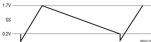
Figure 15. SS in Sustained Hiccup Mode
