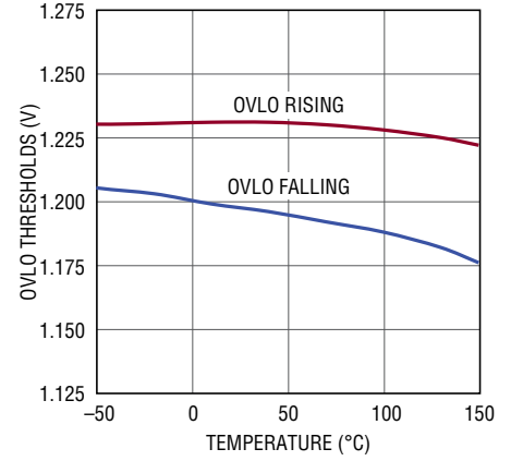
OVLO Thresholds vs Temperature
