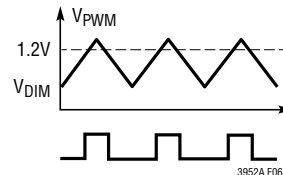
Figure 6. Lower DIM Voltage
