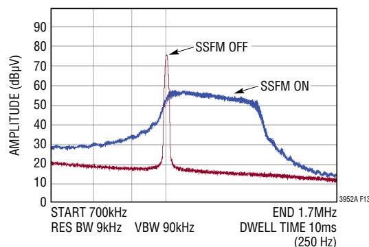
Figure 13. Average Conducted EMI – 1MHz
