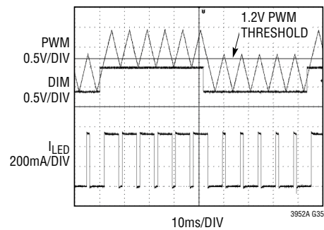
PWM Generator Operation and Step
