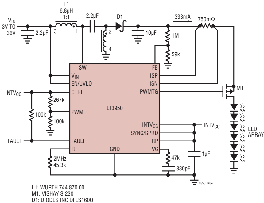
5W SEPIC LED Driver with Internal 10% PWM Dimming
