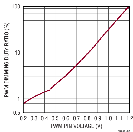
Figure 4. PWM Duty Ratio
