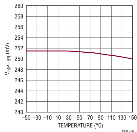
ISP-ISN Threshold (Full Scale) vs Temperature
