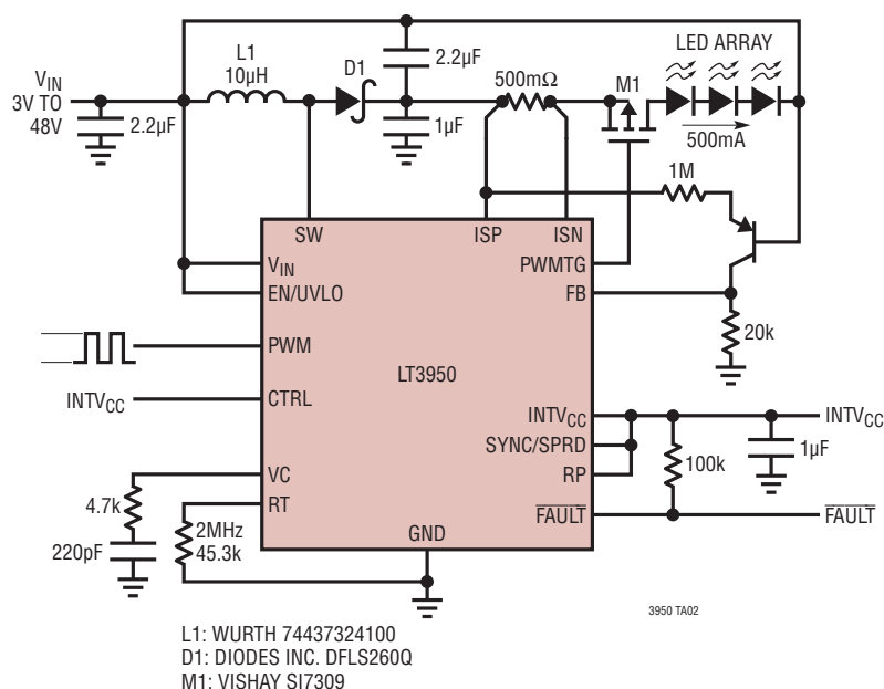
5W Buck-Boost Mode LED Driver with Spread Spectrum Frequency Modulation
