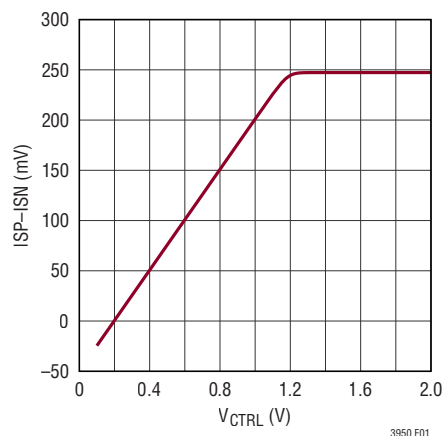
Figure 1. V_{\text{ISP-ISN}} vs CTRL Pin Voltage
