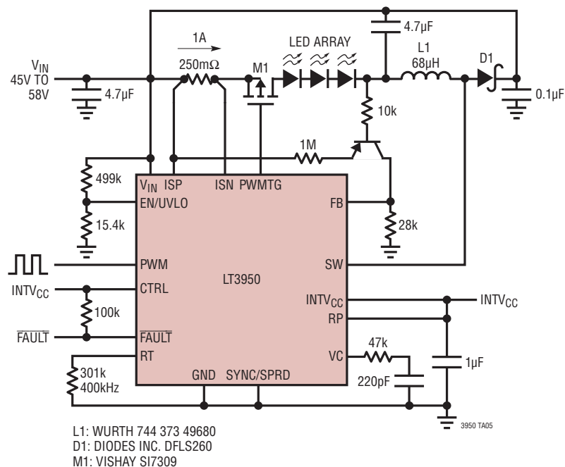
36W Buck-Mode LED Driver
