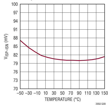
ISP-ISN Threshold (ISP = 0V) vs Temperature
