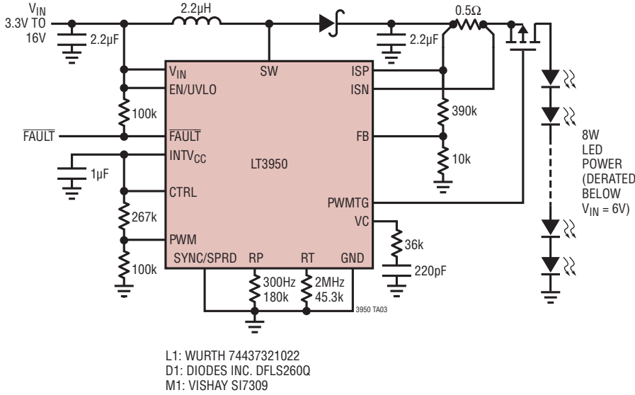
8W Boost LED Driver with Internal 10% PWM Dimming
