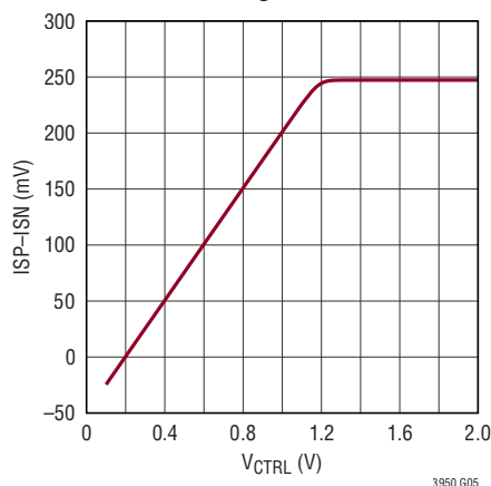
ISP-ISN Full-Scale Threshold vs V_{CTRL} Pin Voltage
