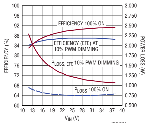
Efficiency and Power Loss with and without PWM Dimming
