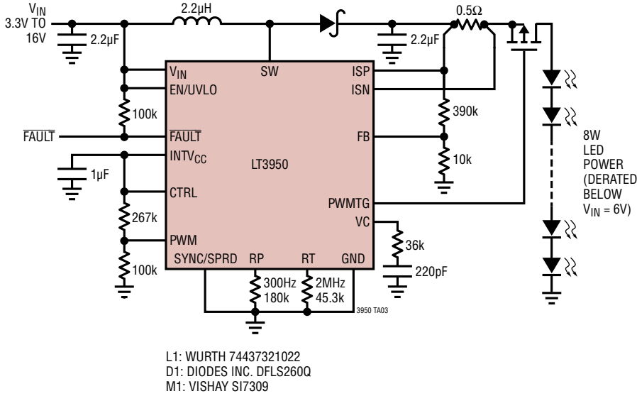
8W Boost LED Driver with Internal 10% PWM Dimming
