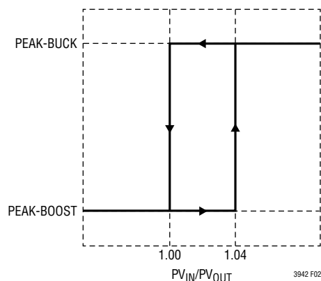
Figure 2. Current Mode vs PV_{IN}/PV_{OUT} Ratio
