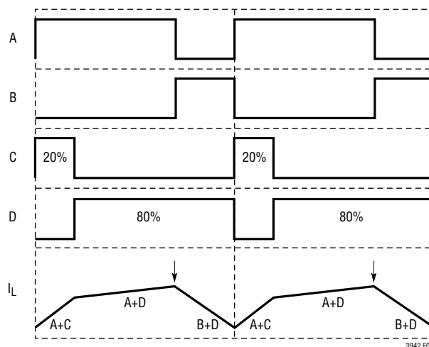
Figure 5. Peak-Buck in Buck-Boost Region ( PV_{IN} \sim PV_{OUT} )
