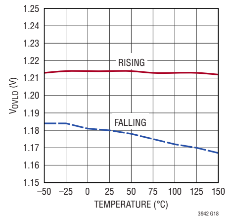
OVLO Threshold
