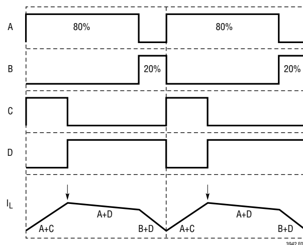
Figure 6. Peak-Boost in Buck-Boost Region ( PV_{IN} \leq PV_{OUT} )
