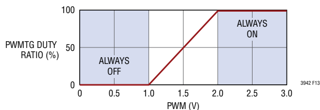
Figure 13. Internal PWM Dimming Duty Ratio vs PWM Voltage
