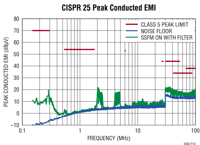
Figure 10. Conducted Peak EMI Comparison
