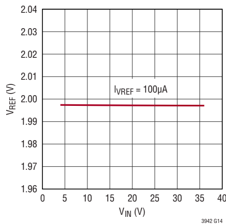
V REF Voltage vs V IN
