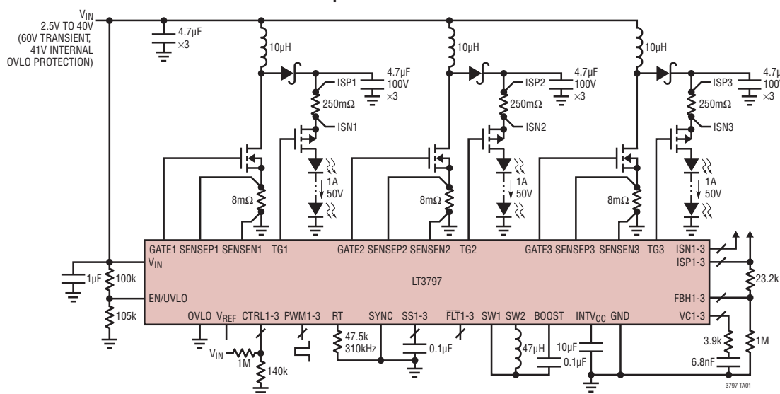
Triple Boost LED Driver
