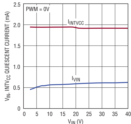
V_{IN} , INTV CC Quiescent Current vs V_{IN}
