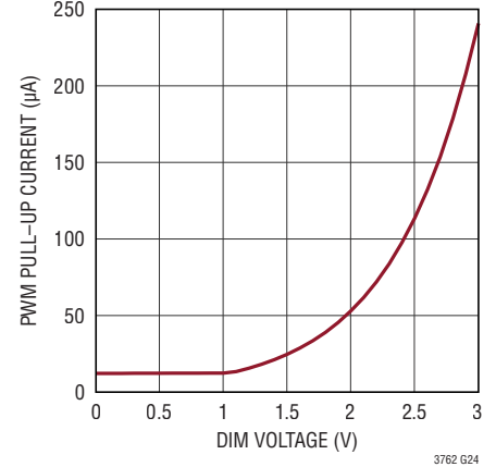
PWM Pull-Up Current vs DIM Voltage
