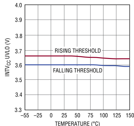
INTV_{CC} Undervoltage Lockout vs Temperature
