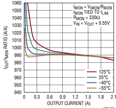
I_{OUT}/I_{MON} Ratio
