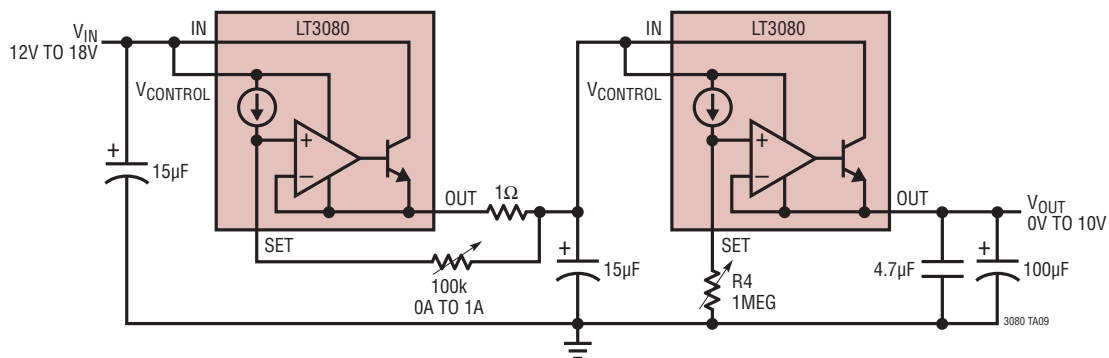
Lab Supply
