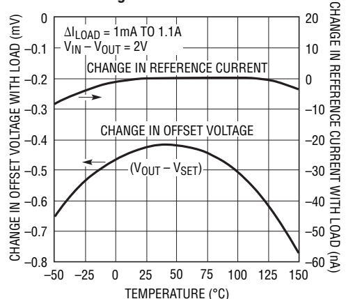
Load Regulation
