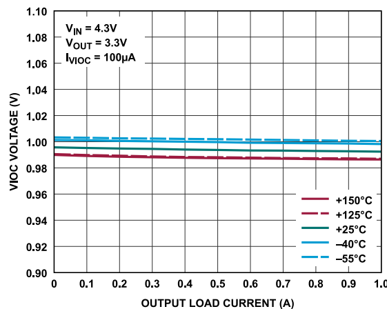
Figure 69. VIOC Voltage vs. Output Load Current
