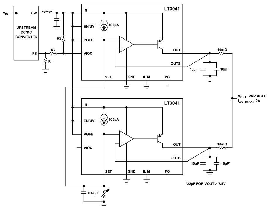
Figure 97. Post Regulating Application with Parallel Devices
