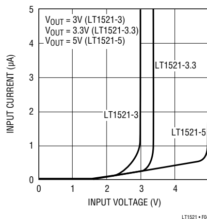
Figure 4. Input Current
