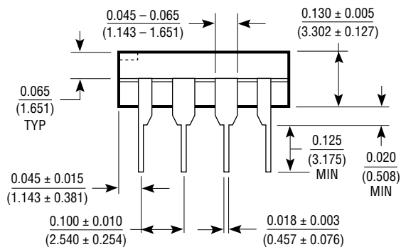
0.300 - 0.320 (7.620 - 8.128) 0.009 - 0.015 (0.229 - 0.381) 0.325 +0.025 -0.015 (8.255 +0.635 -0.381)
