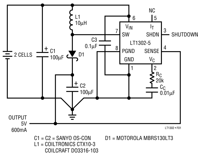
Figure 1. 2-Cell to 5V/600mA DC/DC Converter
