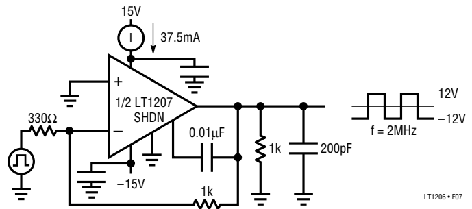
Figure 8. Thermal Calculation Example
