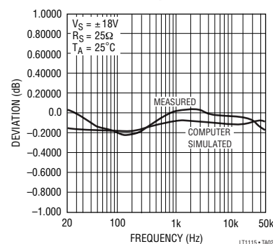
Measured Deviation from RIAA Response. Input at 1kHz = 1mV RMS Pre-Emphasized
