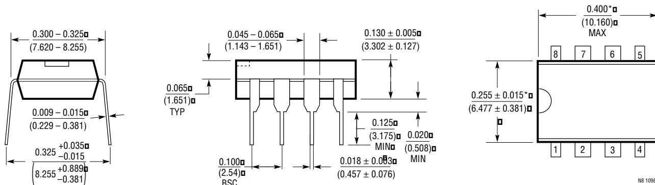
N8 Package 8-Lead PDIP (Narrow 0.300) (LTC DWG # 05-08-1510)
