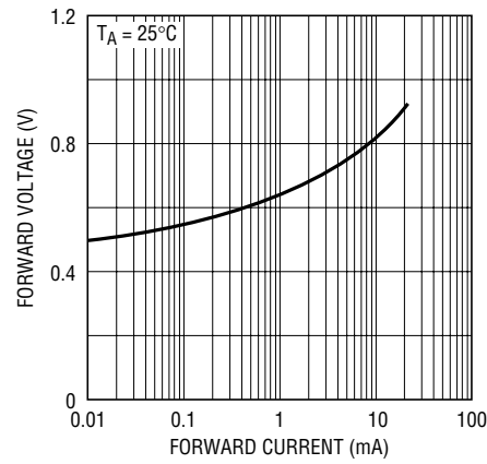
Foward Characteristics
