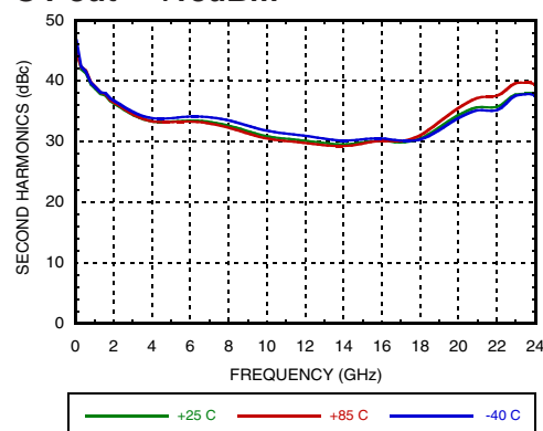
Second Harmonics vs. Temperature @ Pout = +18dBm
