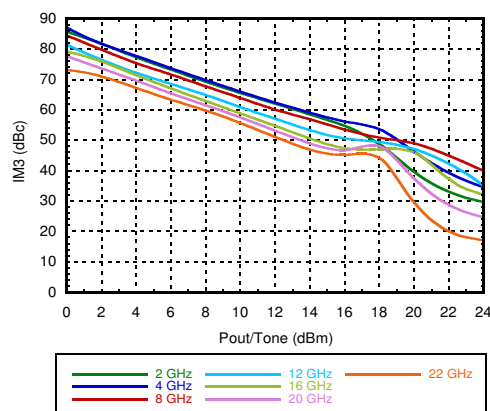
Output IM3 @ Vdd = +12V
