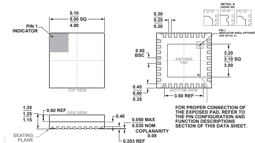
32-Lead Lead Frame Chip Scale Package, Premolded Cavity [LFCSP_CAV] 5mm x 5mm and 1.25mm Package Height (CG-32-2) Dimensions shown in millimeters.
