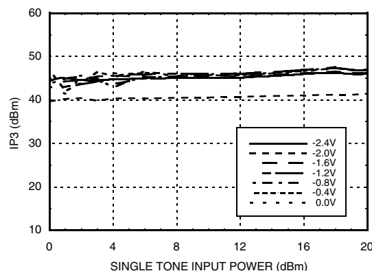
Input IP3 vs. Input Power @ 30 GHz Vctrl2 = Variable, Vctrl1 = 0V
