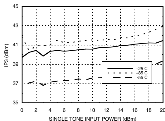
Input IP3 vs Input Power over Temperature @ 30 GHz, Vctrl2 = -2V, Vctrl1 = 0V [1]
