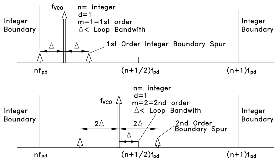
Figure 27. Fractional Spur Example
