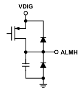
Figure 13. ALMH Interface Schematic (Input)
