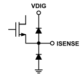
Figure 11. ISENSE Interface Schematic (Input)
