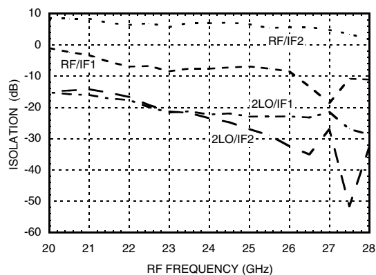
RF/IF and LO/IF Isolations
