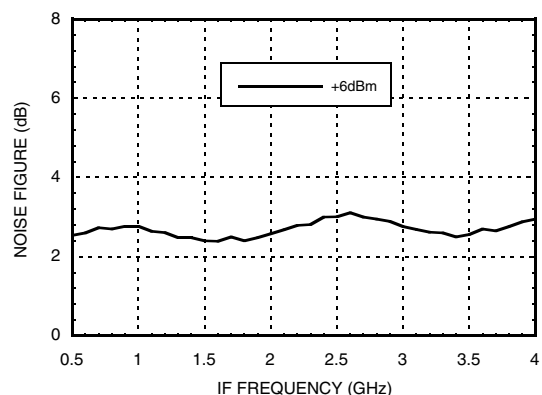
Noise Figure, LO Frequency = 10 GHz
