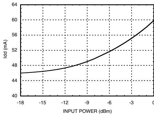
Current vs. Input Power @ 16 GHz
