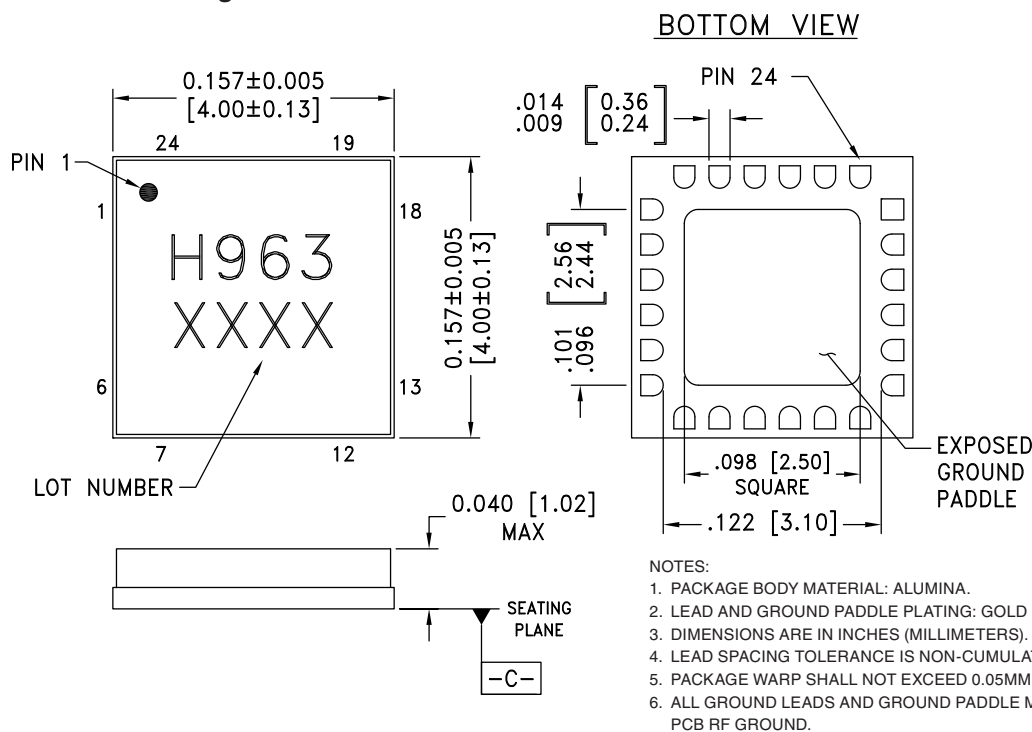
Outline Drawing
